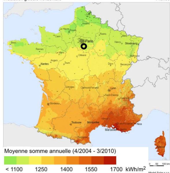
Irradiation globale horizontale France
